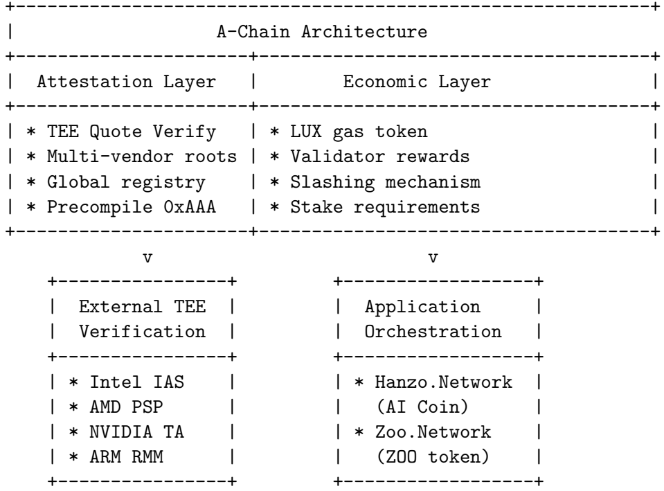
Figure 1: A-Chain architectural layers
