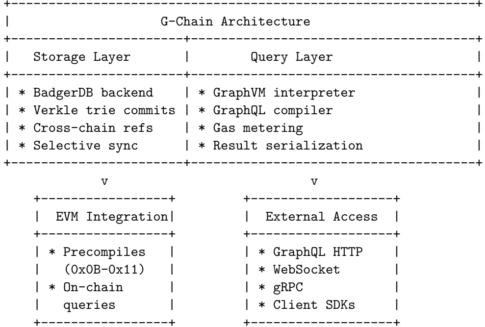
Figure 1: G-Chain architectural layers
