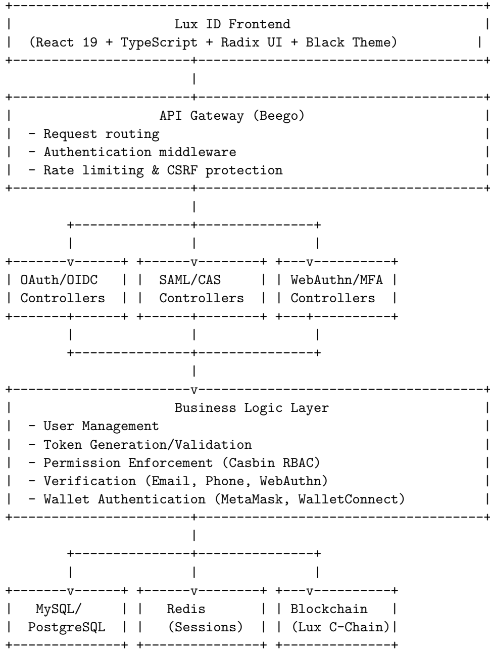
Figure 1: Lux ID System Architecture
