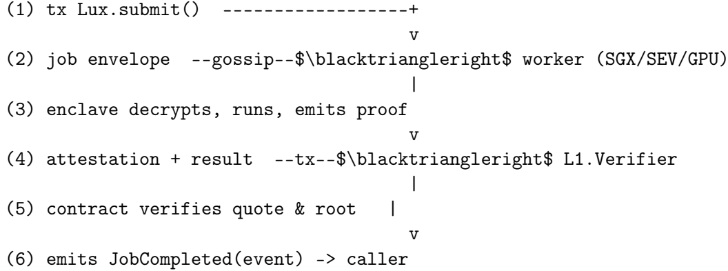
Figure 1: Lux TEE Mesh data flow
